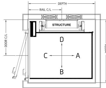
Single Opening Rail Left, Right Hand Door / Rail Right, Left Hand Door
